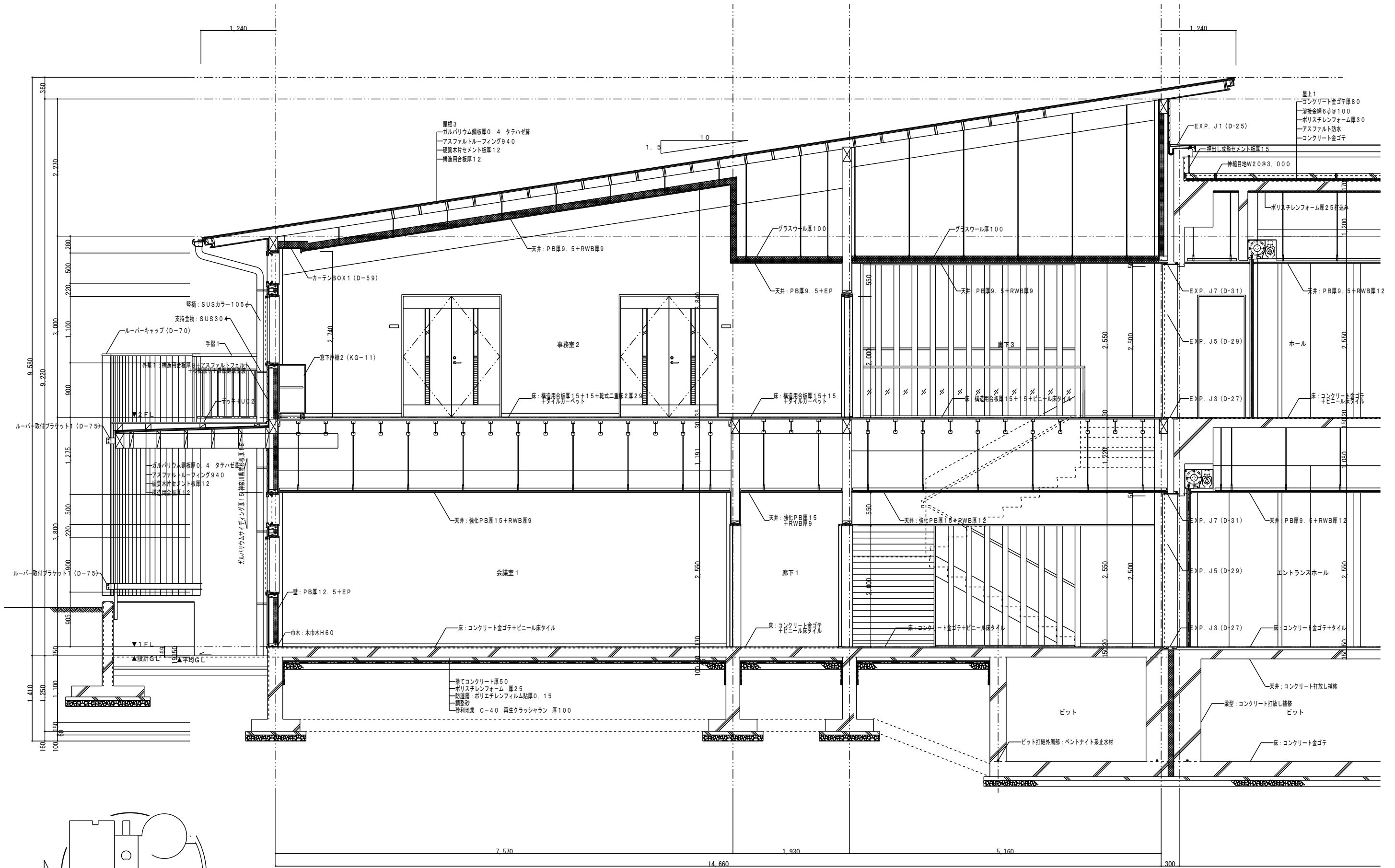
矩計図-1 1:30
