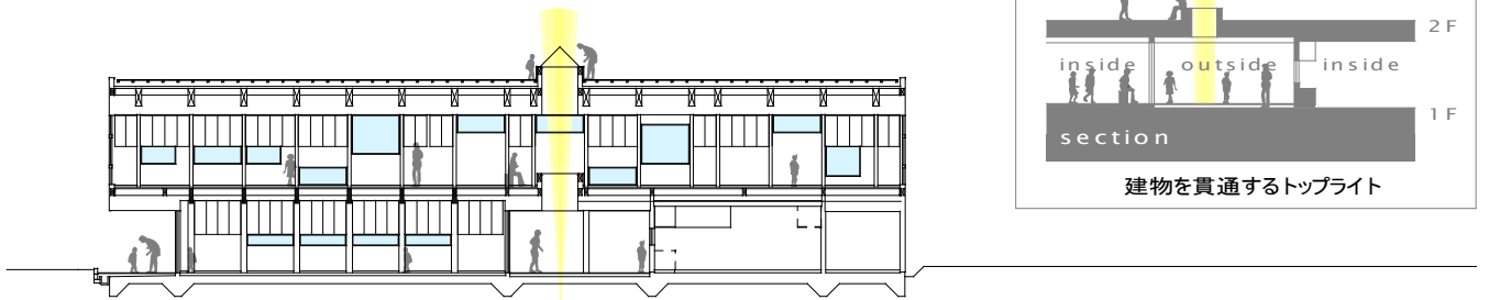
b-b section
